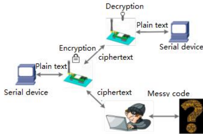
Figure 10 Data security
