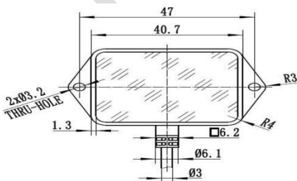
Figure 1. Front view of HPS-167S-L
