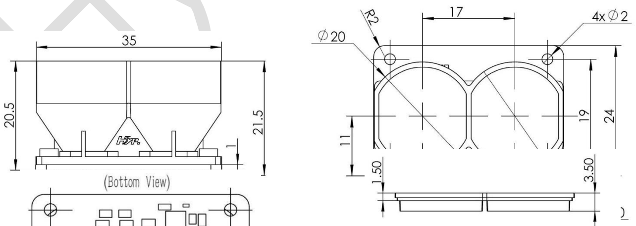
Figure 1. Front view of HPS-167-L
