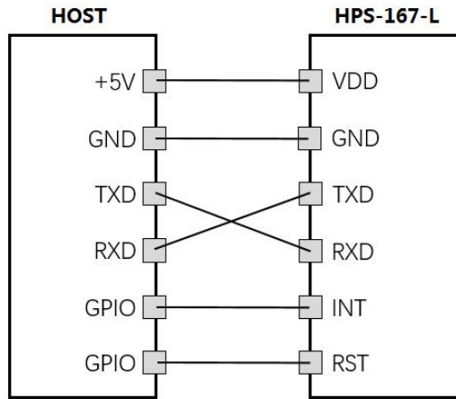
Figure. 6 Application schematic of the HPS-167-L
