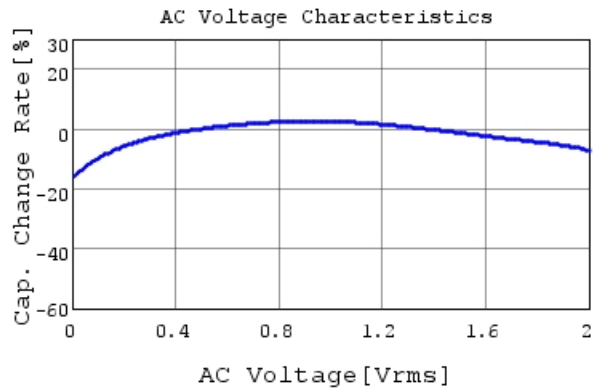
GRM022R60J104ME15 C-AC Voltage capchange, Dc
