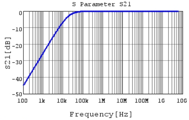
GRM022R60J104ME15 S21 DC0V, 25degC
