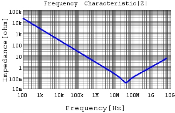
GRM022R60J104ME15 |Z| DCOV, 25degC
