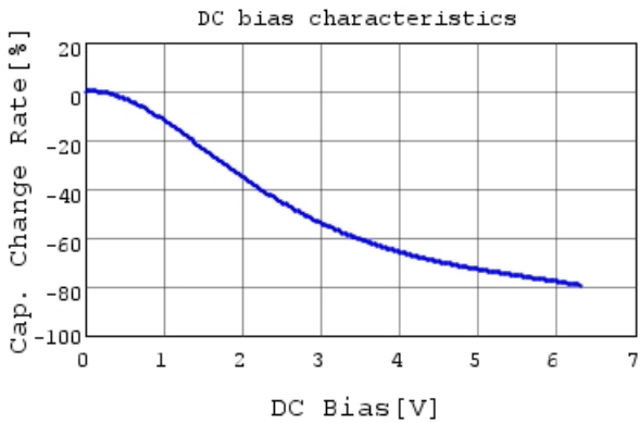
GRM022R60J104ME15 C-DC bias capchange, 25.0c
