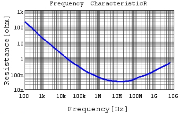
GRM022R60J104ME15 R DCOV, 25degC
