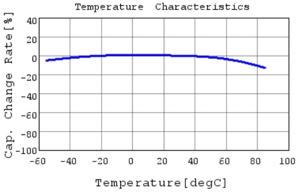
GRM022R60J104ME15 C-Temp. capchange, DC0.0V,
