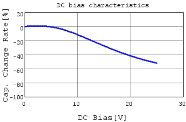
GCM32ER71E106KA57 C-DC bias capchange, 25.0c
