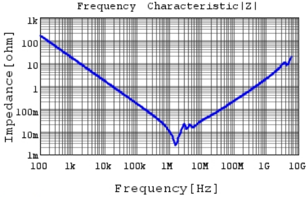
GCM32ER71E106KA57 |Z| DCOV, 25degC
