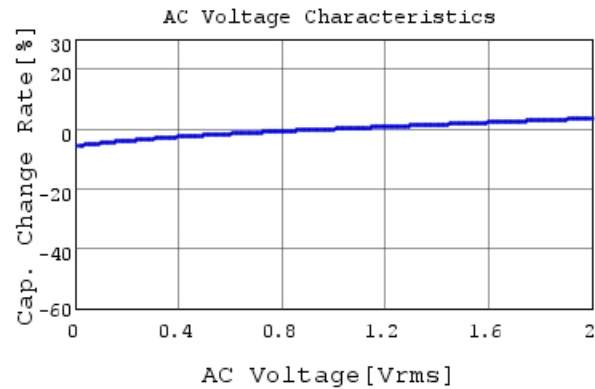
GCM32ER71E106KA57 C-AC Voltage capchange, Dc
