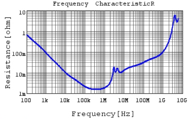
GCM32ER71E106KA57 R DCOV, 25degC
