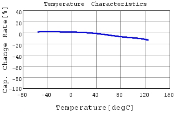
GCM32ER71E106KA57 C-Temp. capchange, DC0.0V,
