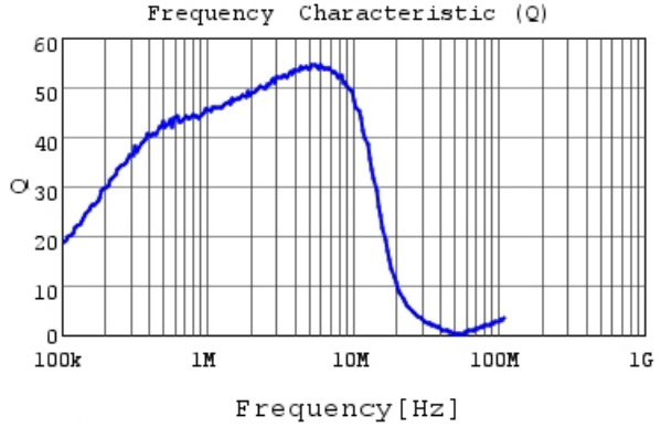
LQM2HPN2R2MG0 Q
