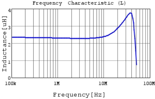
LQM2HPN2R2MG0 L
