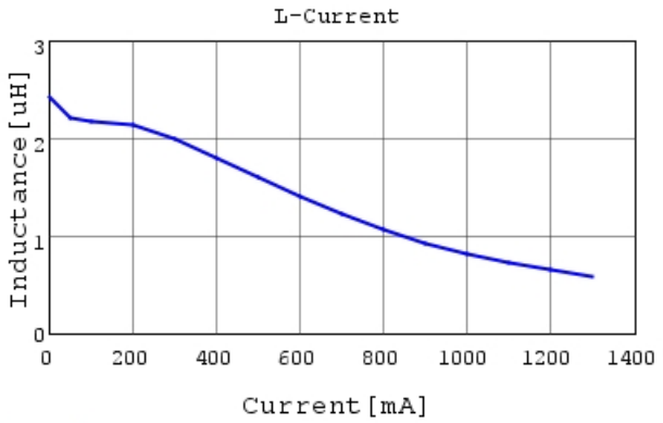
LQM2HPN2R2MG0 L-Current 20degC
