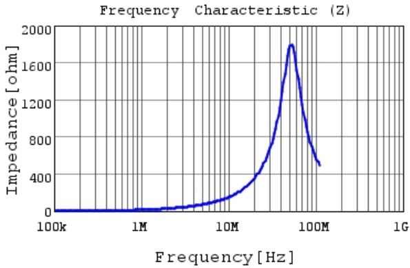
LQM2HPN2R2MG0 |Z|
