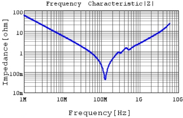
GRM2165C1H272JA01 |Z| DCOV, 25degC
