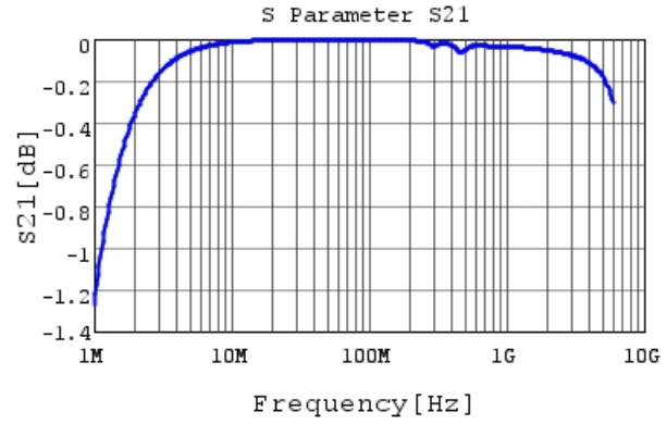
GRM2165C1H272JA01 S21 DCOV, 25degC
