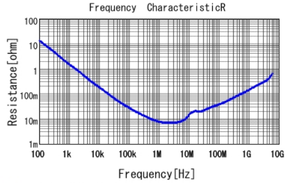
■ GRM155C71A225KE11 R DCOV, 25degC
