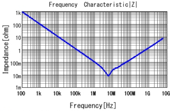
■ GRM155C71A225KE11 |Z| DCOV, 25degC
