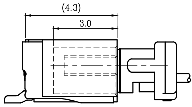
MATED CONDITION
