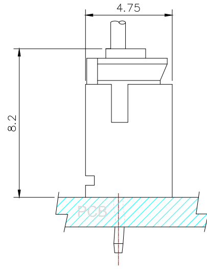
ASSEMBLY LAYOUT
