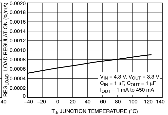
Figure 12. Load Regulation vs. Temperature – V_{OUT} = 3.3\text{ V} (WLCSP4)
