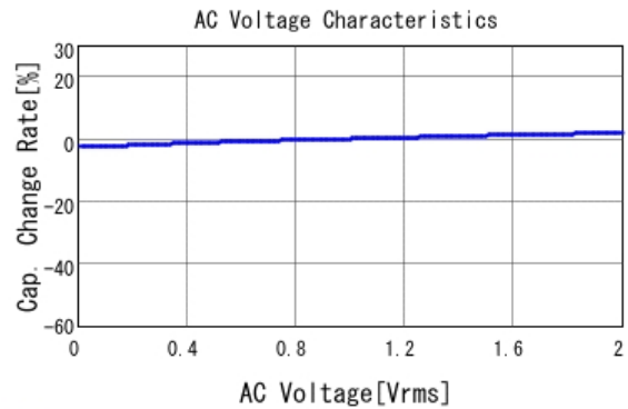
■ GRM155C71H104KE19 C-AC Voltage capchange, DCOV, 25.0d
