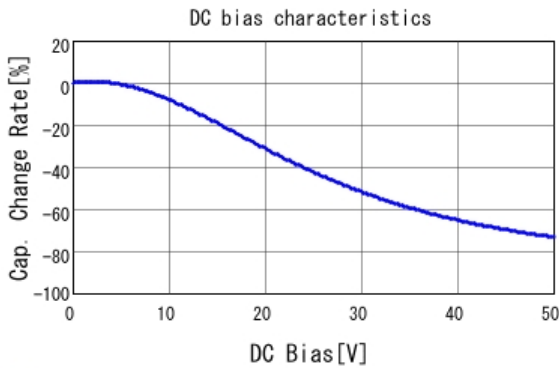
■ GRM155C71H104KE19 C-DC bias capchange, 25.0degC, AC1.
