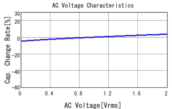
■ GCJ32DC72A475KE01 C-AC Voltage capchange, DC0V, 25.0d
