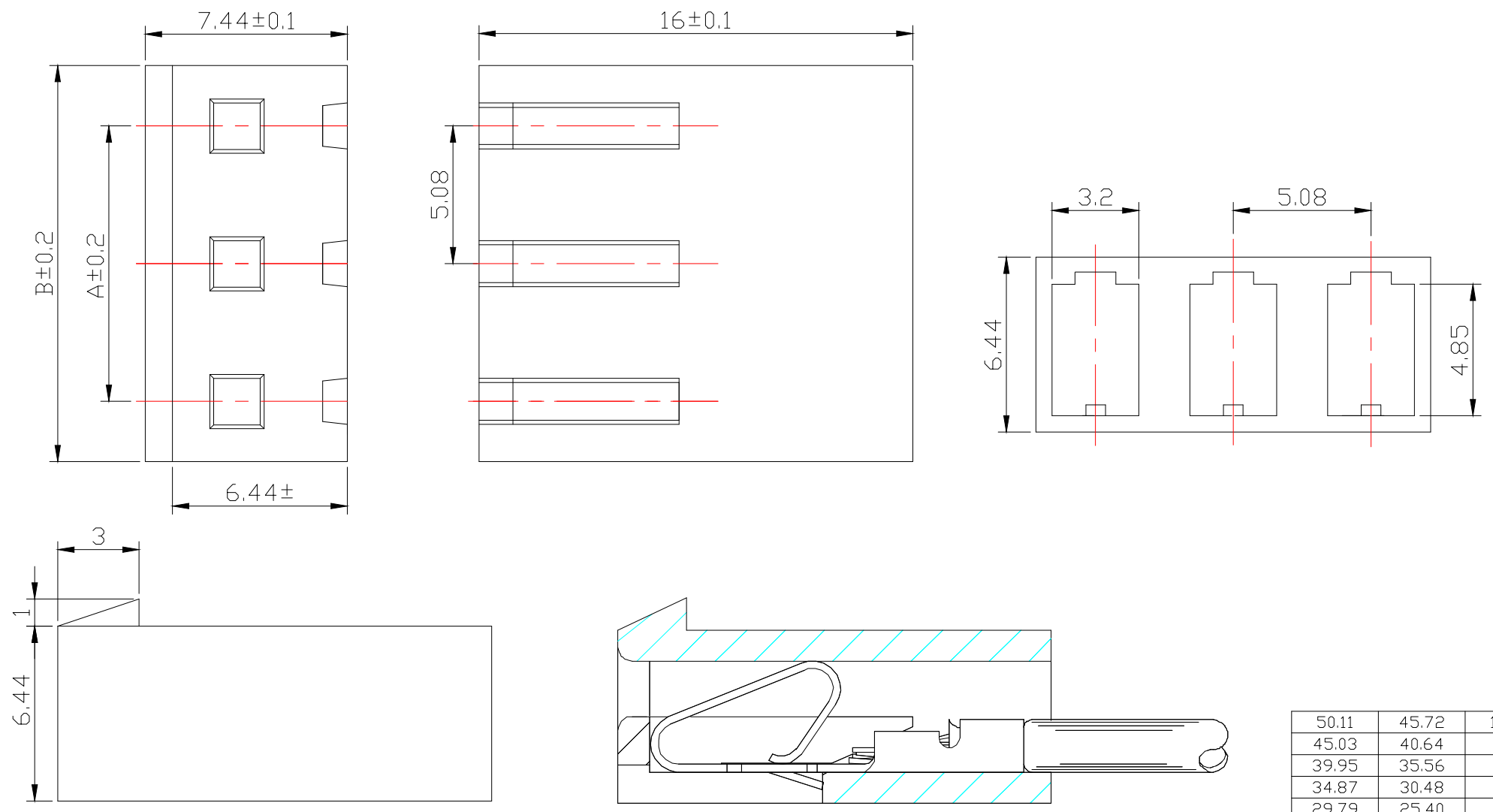
SECTIONAL DRAWING
