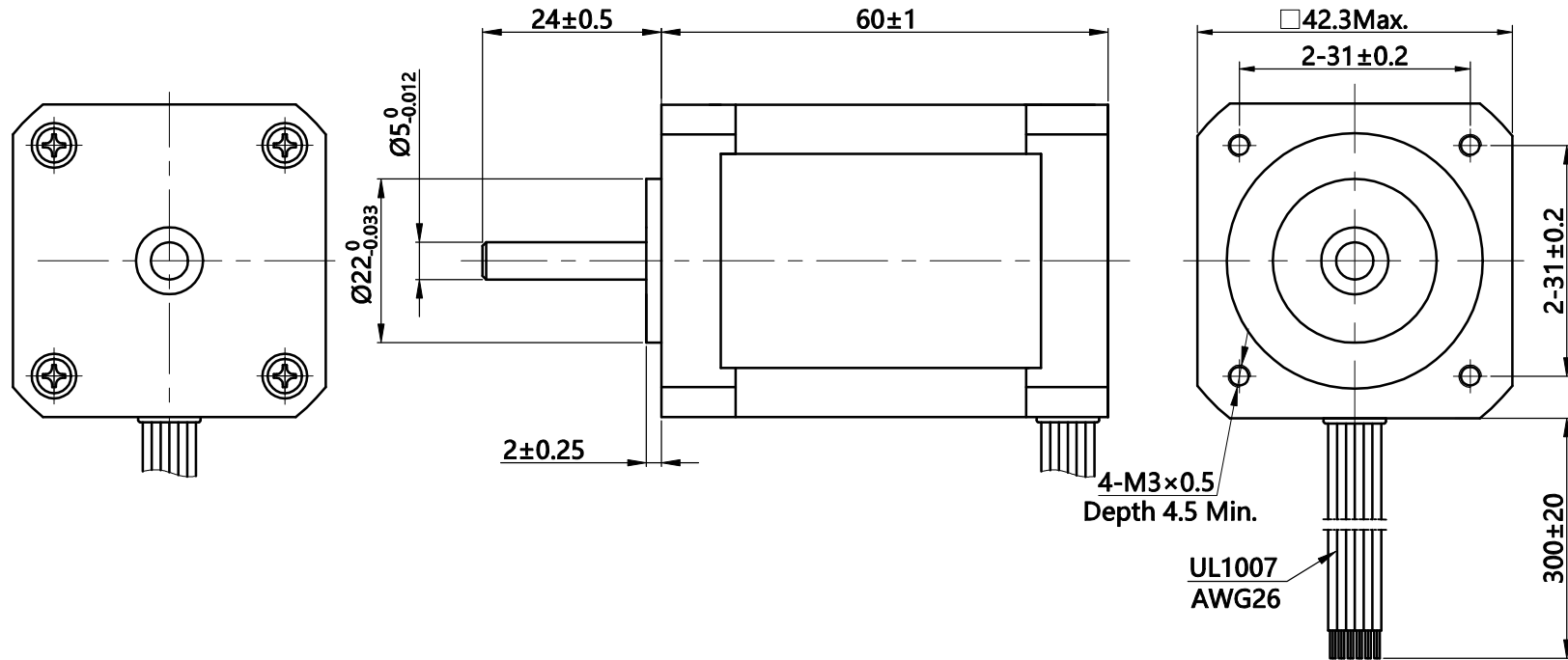
Clockwise view from mounting side
