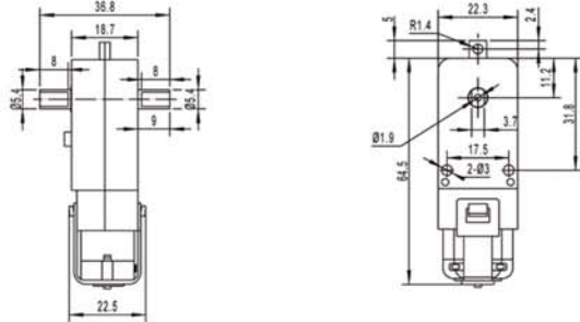
Gear Motor Dimensions (mm)
