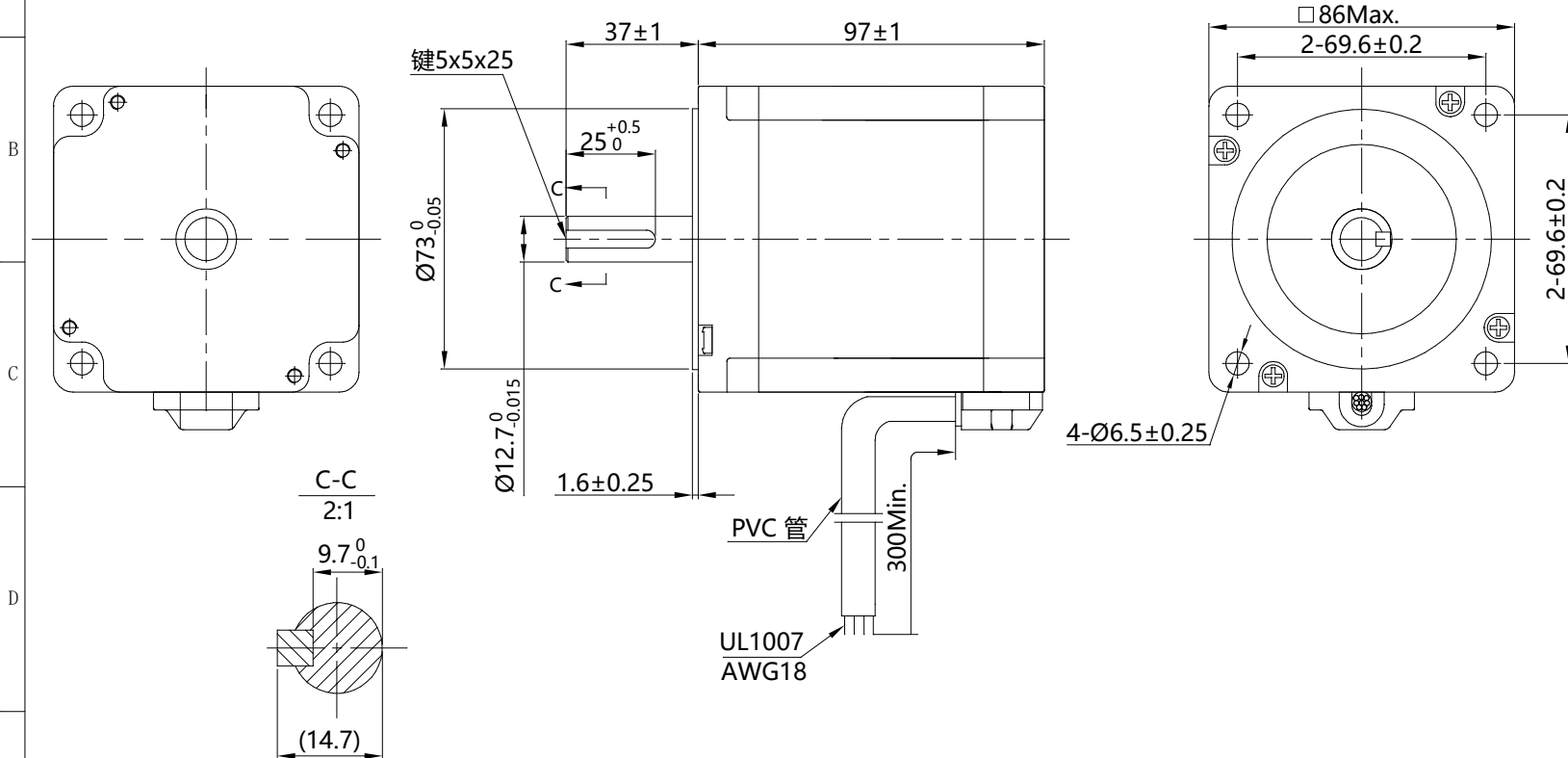
外形图 (DIMENSIONS) unit=mm
