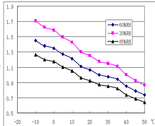
Fig4.Typical temperature/humidity characteristics
