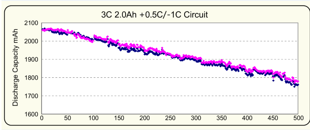
Discharge Capacity vs Cycle Life Graph for 2 Sample Batteries
